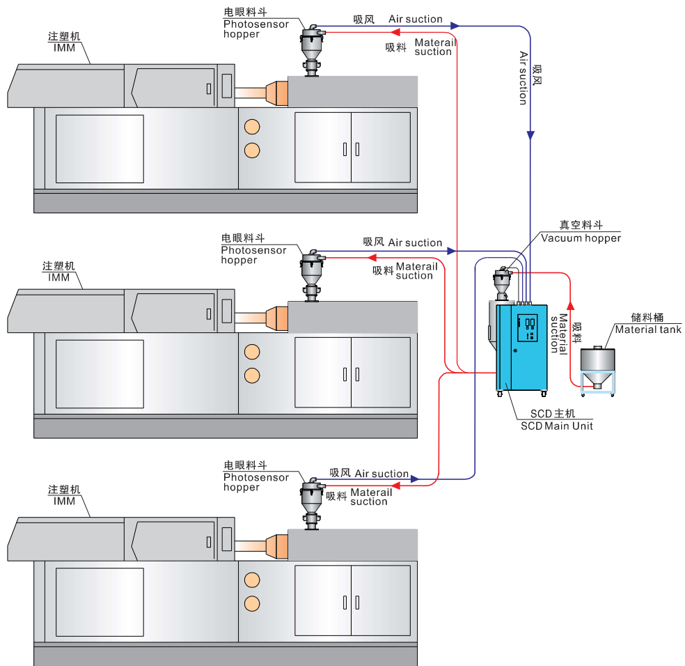
1对3 四段送料示意图 (选配) For Serving Three Machines: Four-stage Conveying System (Optional)
