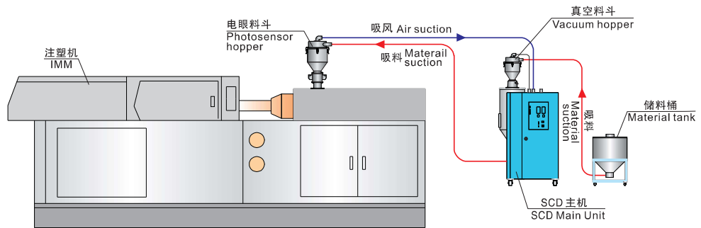
1对1 二段送料示意图 (标准) For Serving One Machine: Two-stage Conveying System (Standard)
